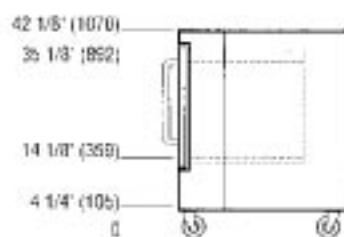
BP-50 SIDE VIEW WITH CASTERS
