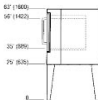
BP-50 SIDE VIEW WITH 25° LEGS
