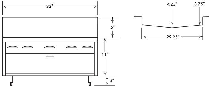
Model 2932SF front view
