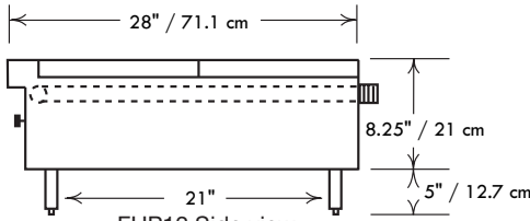
FHP12 Side view
