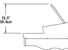
LID HEIGHT DETAIL ALL MODELS
