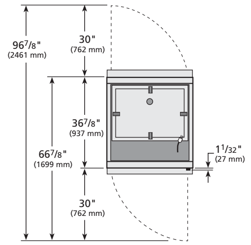
PLAN VIEW
