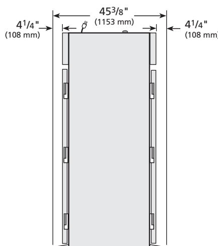
RIGHT VIEW
