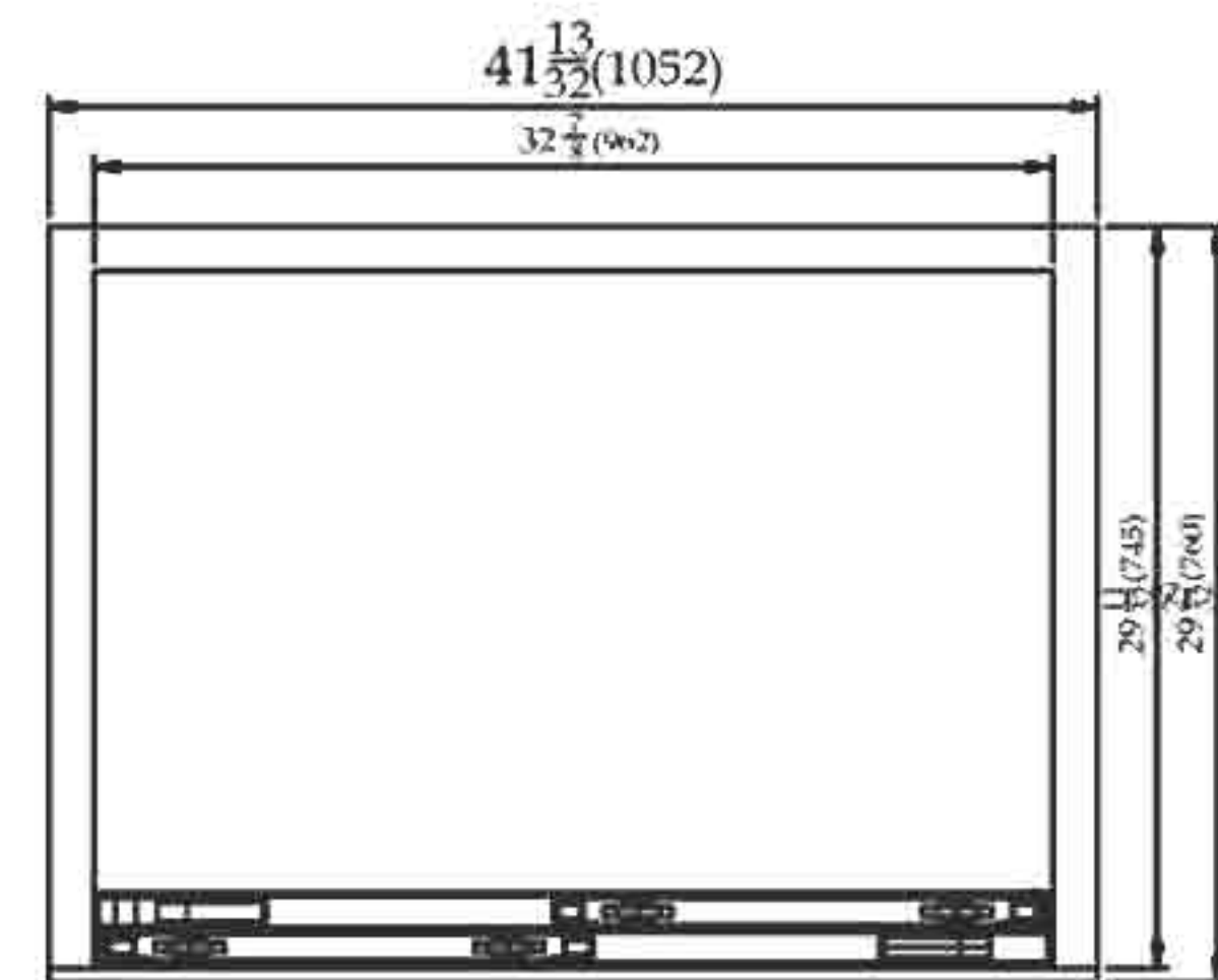
TGM-35R PLAN VIEW
