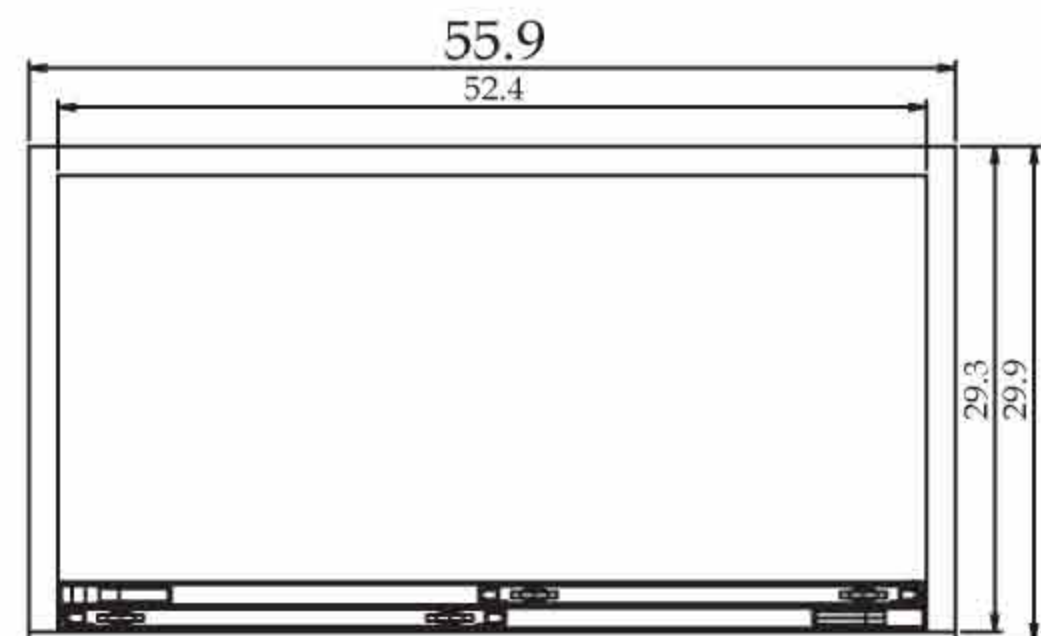
TGM-48R PLAN VIEW
