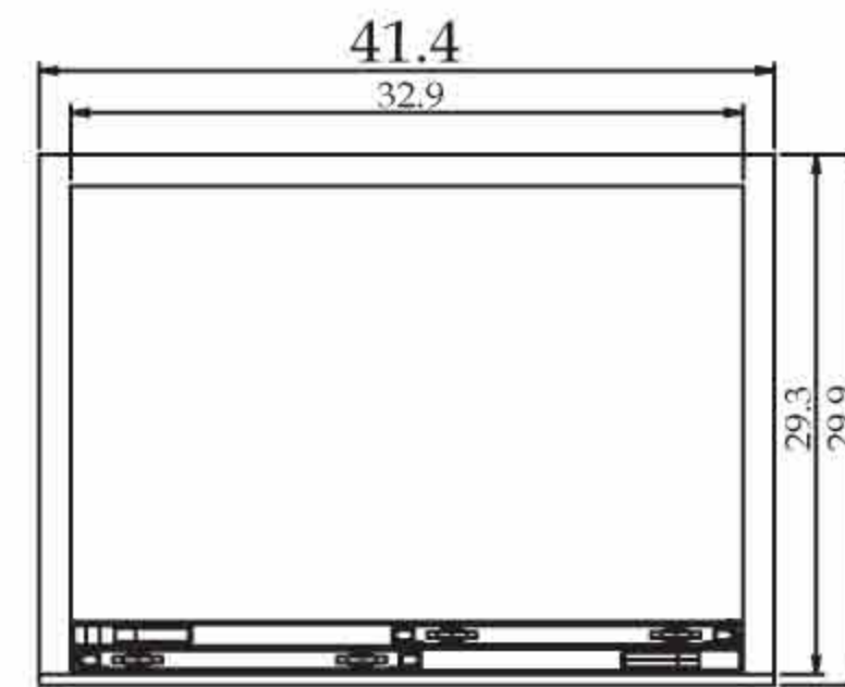
TGM-35R PLAN VIEW
