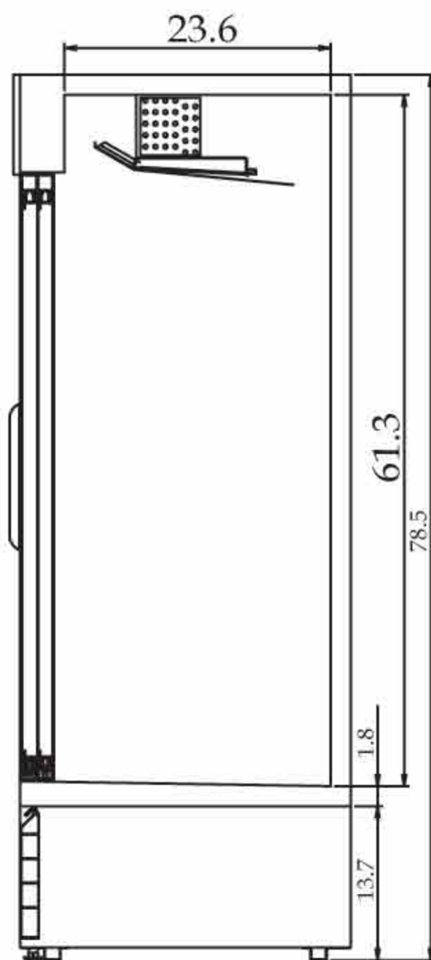
TGM-35R/48R SIDE VIEW
