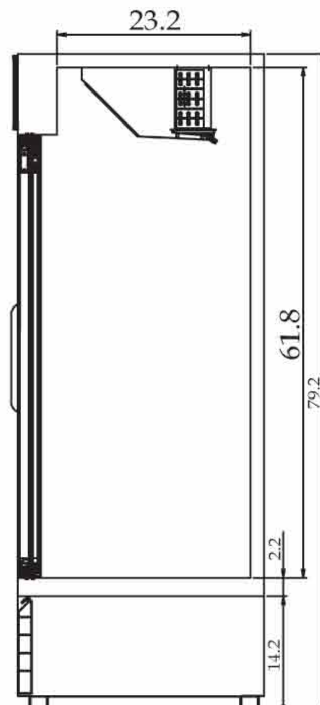
TGM-69R SIDE VIEW
