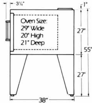
ECCO-T on Fabricated 27" legs
