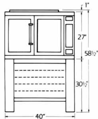
ECCO-T on Fabricated Rack-Holder Base (LS-F11RS)
