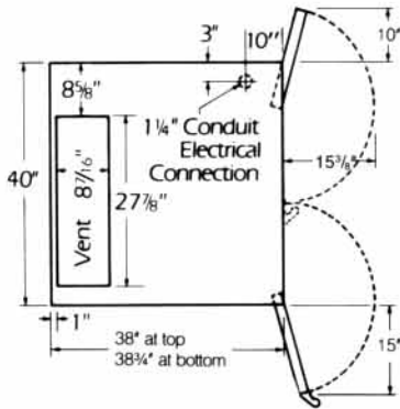
PLAN VIEW
