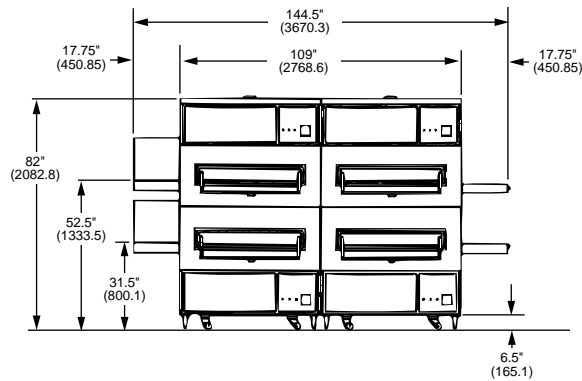
FRONT VIEW - PS360T-D
