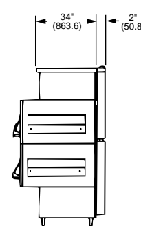
SIDE VIEW - PS360T-D
