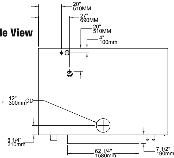
Iso View
